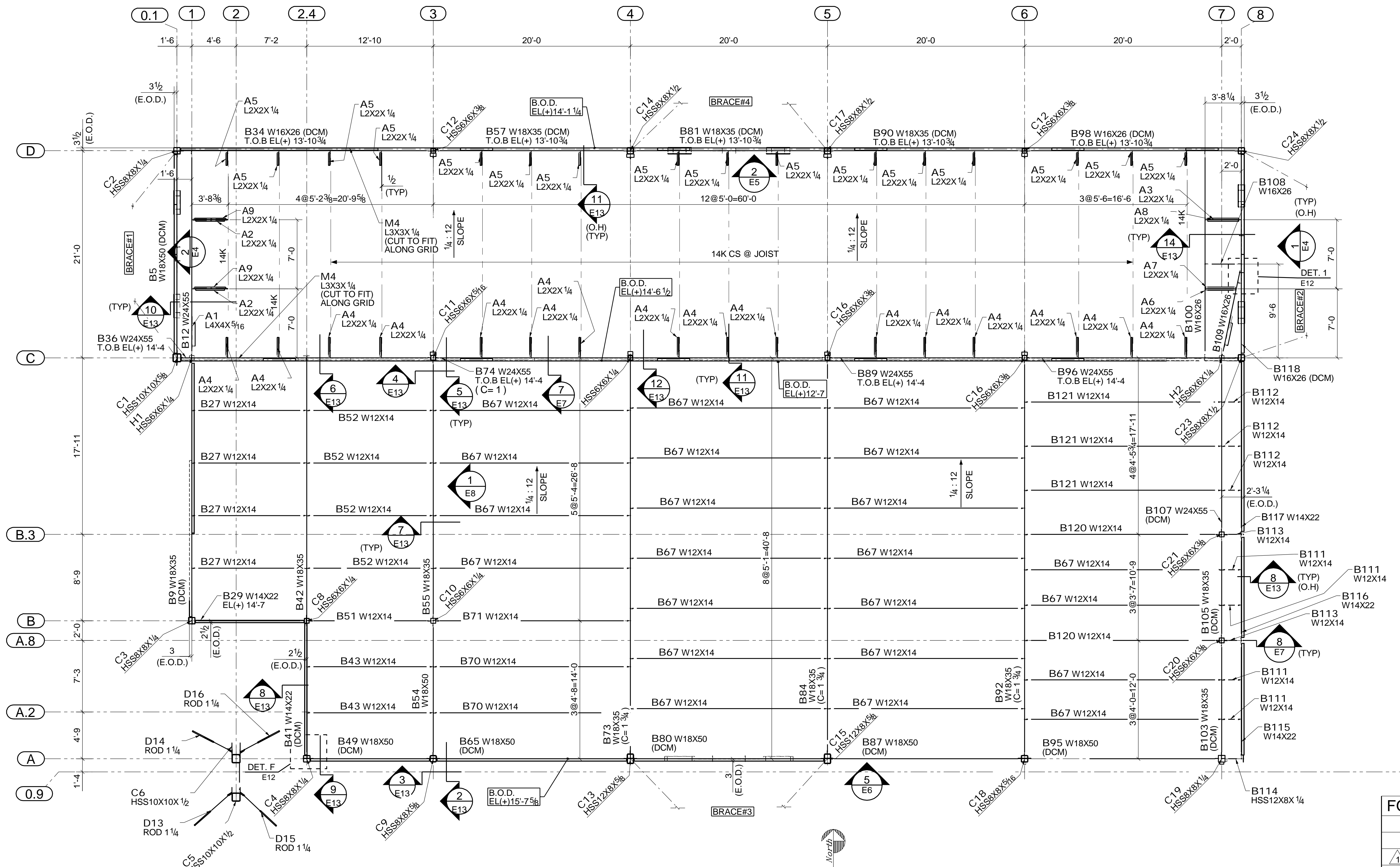
ROOF FRAMING PLAN (REFER: 1/S1.3)
