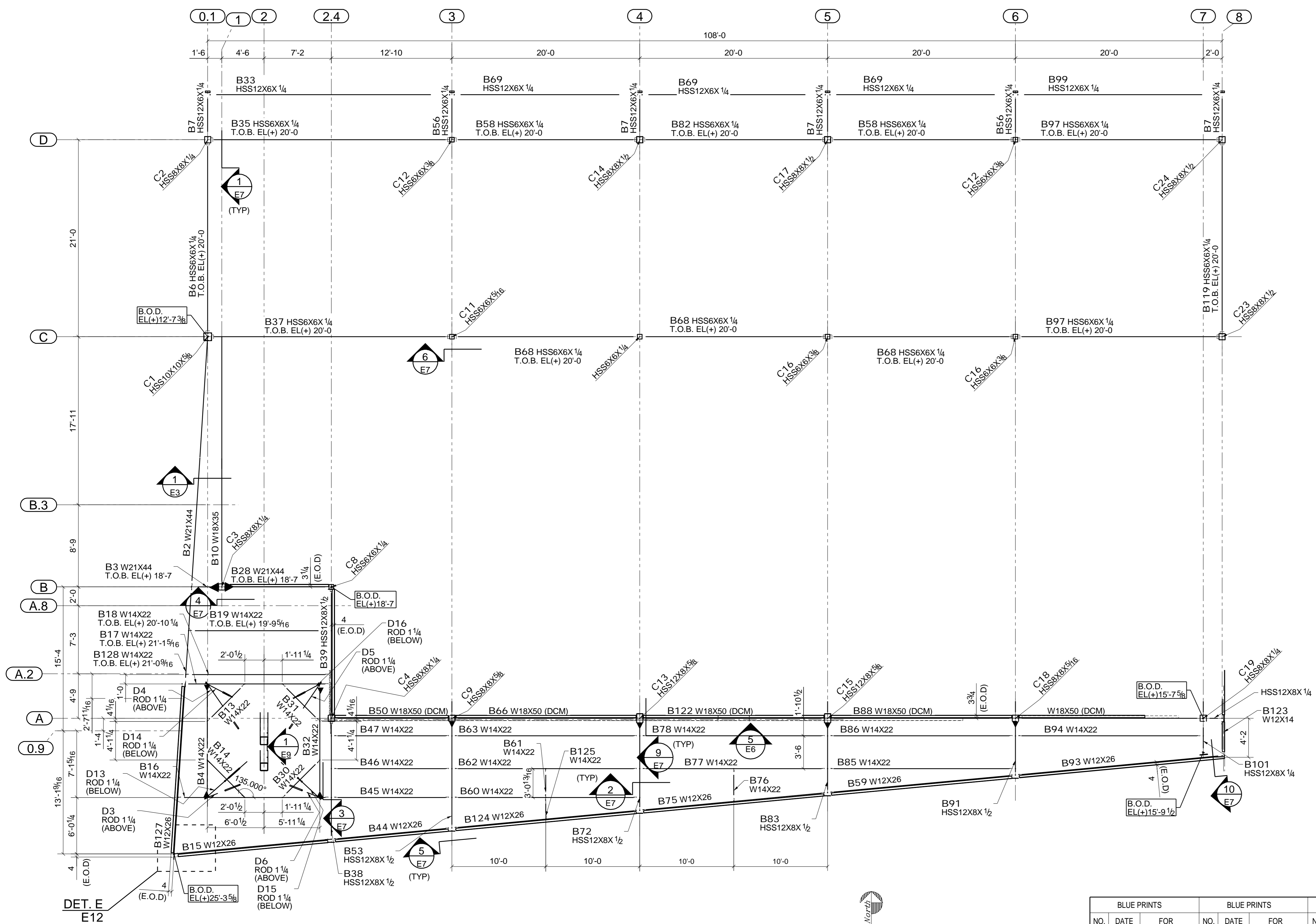
KITCHEN PARAPET & FRONT CANOPY FRAMING PLAN (REFER: -1/S1.4)
