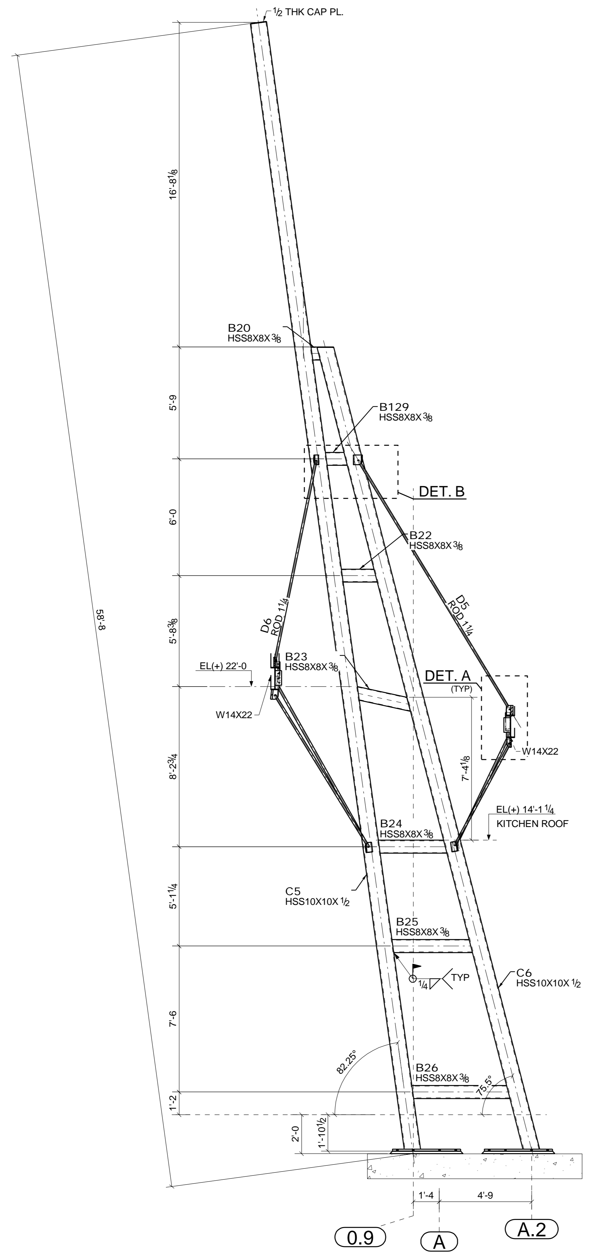
1 MAIN SPIRE ELEVATION (REFER:-1/S2.2)
