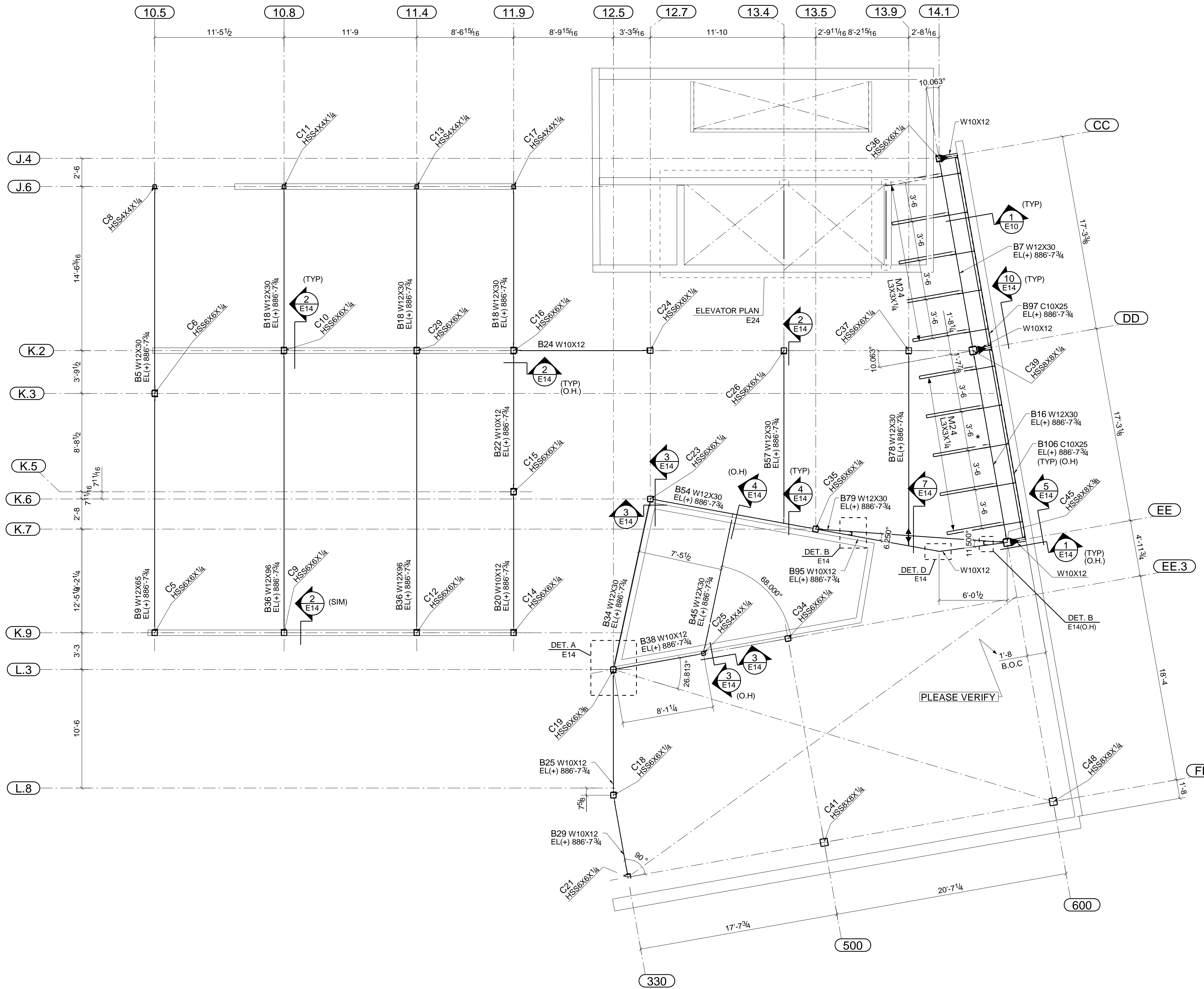
SIXTH FLOOR FRAMING PLAN(SEGMENT 1) (REFER:-S7.1.6.0)
